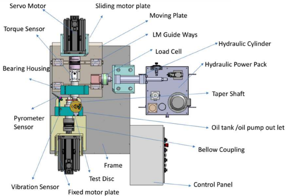
Conceptual drawing of the twin-disc tribometer test rig
